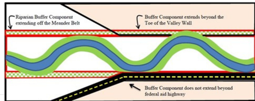
FIGURE 4: RIVER CORRIDORS
