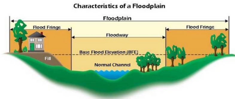
FIGURE 3: TYPICAL FLOODPLAIN
